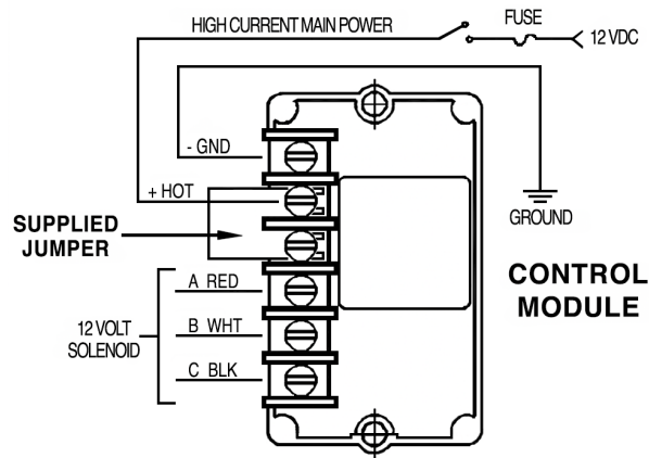
Figure 1 12 VOLTS
