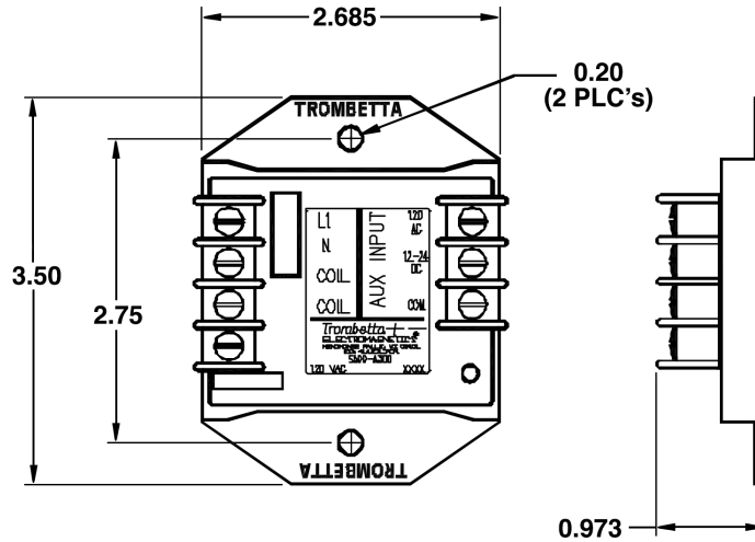
FIGURE #1 120 VAC AUX CONTROL
