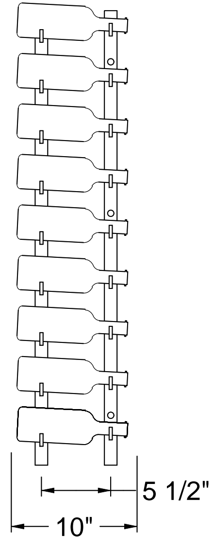
(Mounting for Splits) Front View
