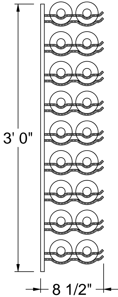
(Standard Mounting) Side View
