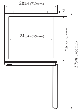
PLAN VIEW
