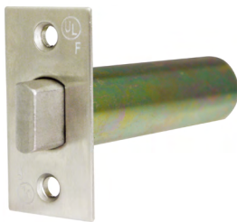
LSL08N 5" Spring Latch 1-1/8" Faceplate CL/CK Series
