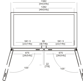
C-49RM TOP VIEW
